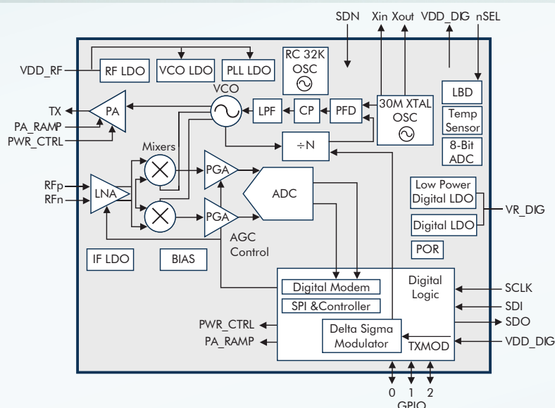
Si4432 BLOCK DIAGRAM
